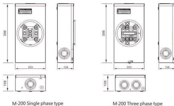
M-200 Single phase type
